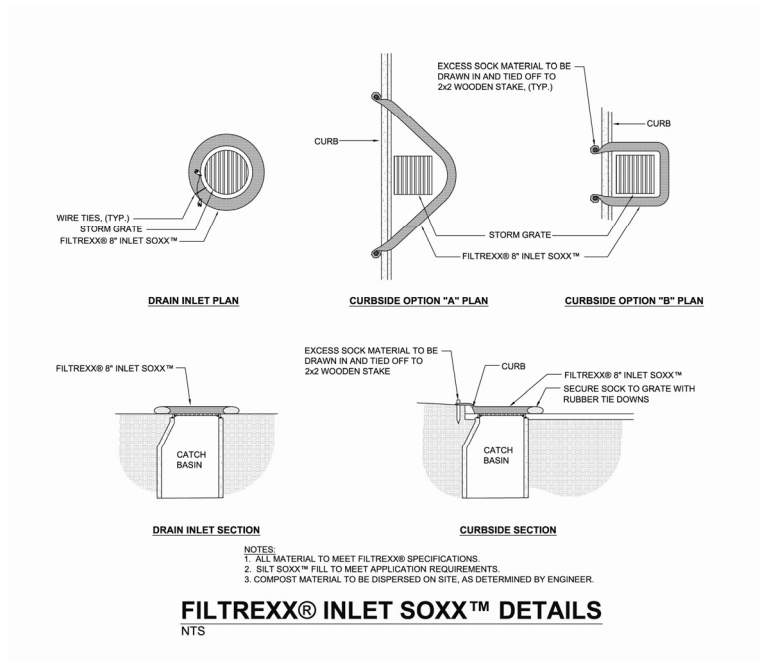
Figure 2.2. Engineering Design Drawing for Curb Sediment Containment InletSoxx™
