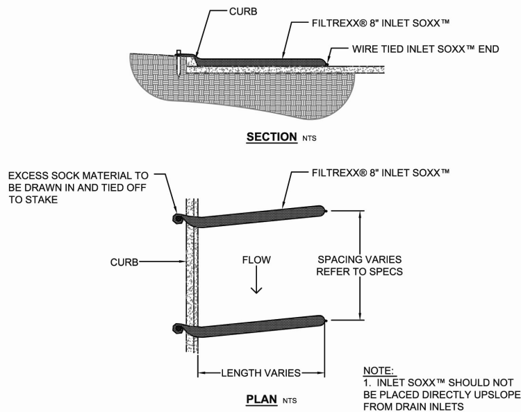
Figure 2.2. Engineering Design Drawing for Curb Sediment Containment InletSoxx™
